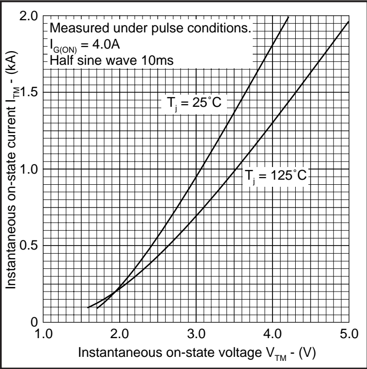
Fig.2 On-state characteristics
