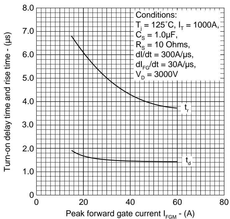
Fig.14 Delay time &amp; rise time vs peak forward gate current
