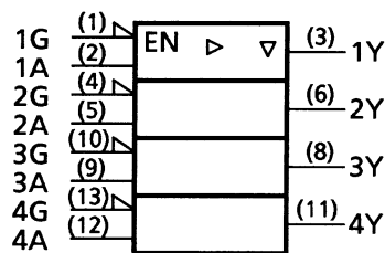
TC74HC126A
