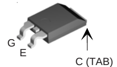
PLUS220SMD (IXGV...S)
