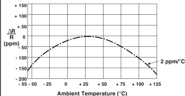
FIGURE 4 - TYPICAL RESISTANCE/ TEMPERATURE CURVE
