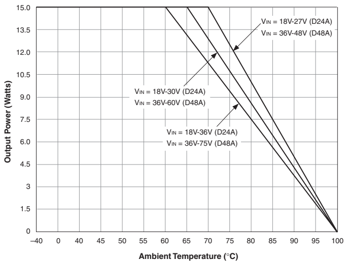
D24A and D48A Temperature Derating for 2.5V/5V/12V/15V Output Models
