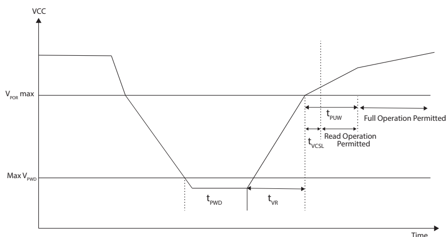
Figure 16-1. Power-Up Timing
