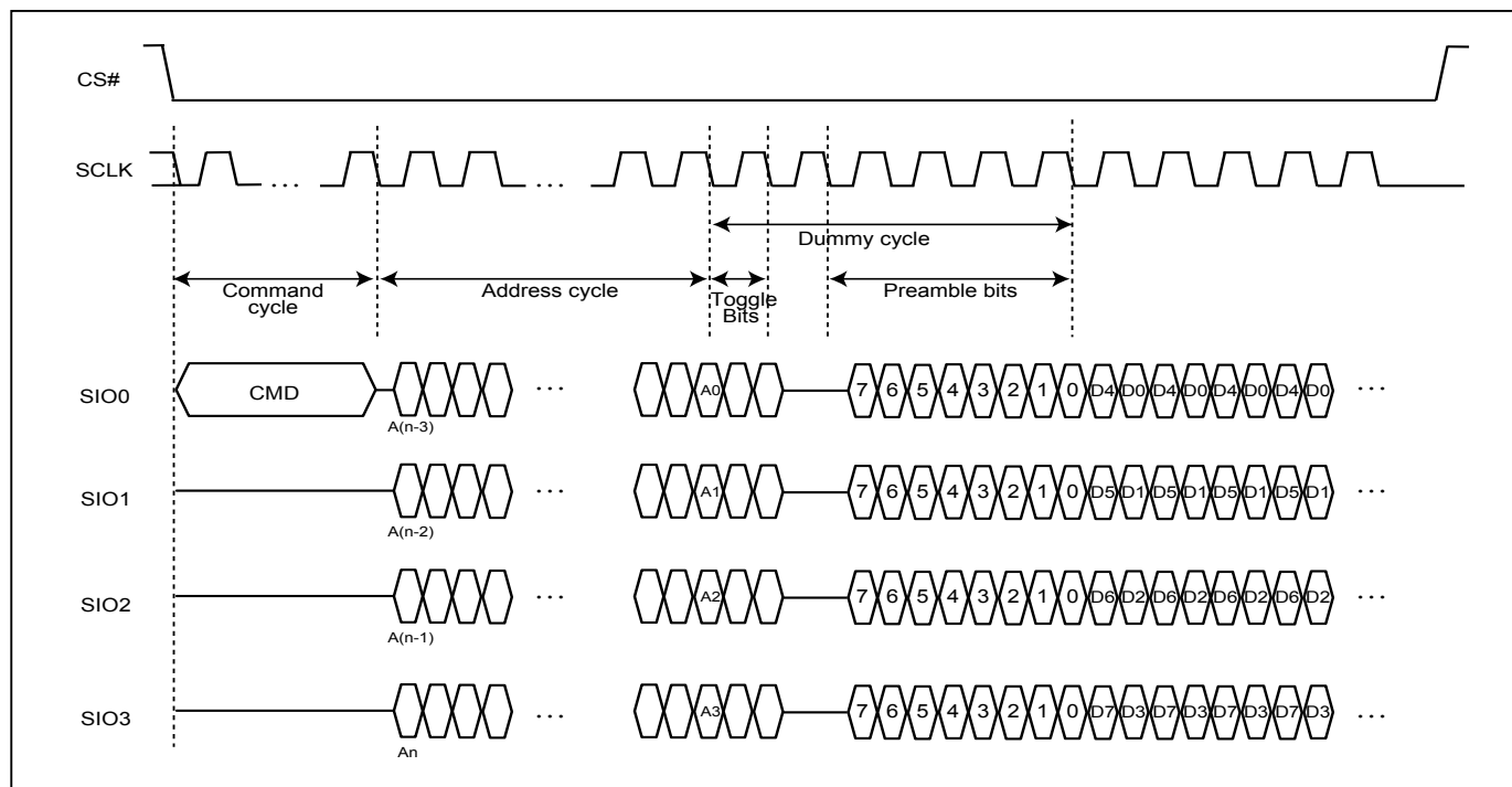
Figure 54. DTR4IO (DC=6)
