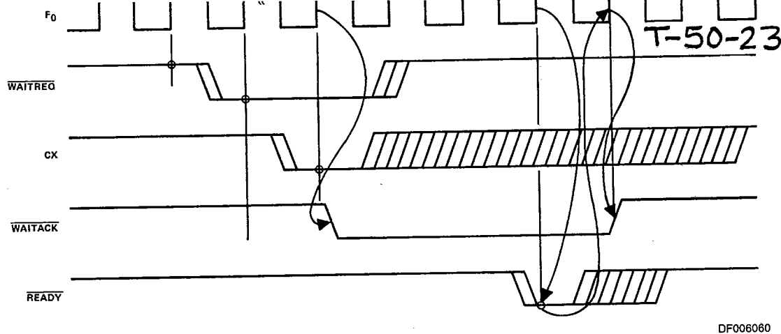
Figure 9. Am2925/Am2925A WAIT/READY Timing
