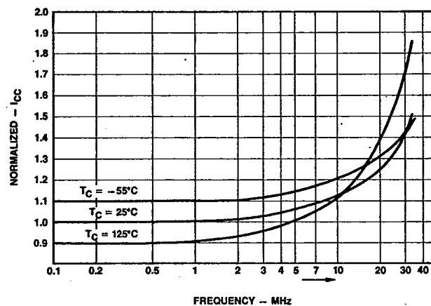
Figure 14. Am2925 I_{CC} Normalized vs Frequency ( V_{CC} = 5.5 V)
