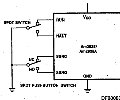
Figure 6. Switch Connection for RUN/HALT and Single Step
