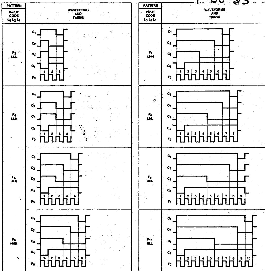
Figure 7. Am2925/Am2925A Clock Waveforms
