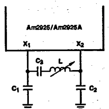
Figure 4. L-C Tuned Oscillator
