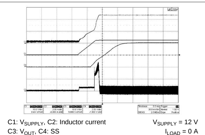
Figure 48. Start-Up
