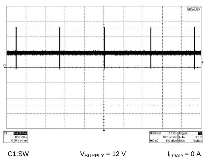
Figure 46. Skip Cycle
