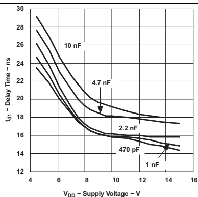
Figure 15. Delay Time ( t_{D1} ) vs Supply Voltage (UCC27423)
