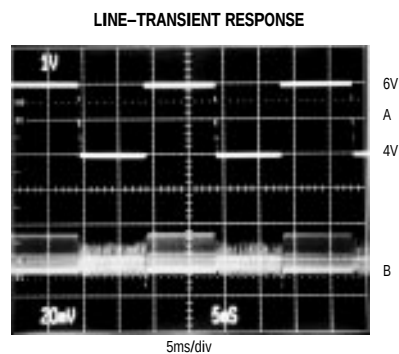
A: V_{IN} (4V to 6V) B: V_{OUT} , AC COUPLED, 20mV/div I_{OUT} = 50mA , V_{OUT} = 12V
