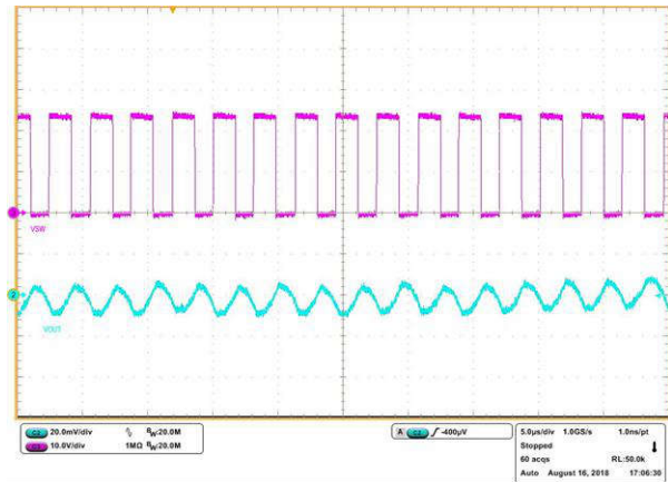
Figure 7-15. Full-Load Switching
