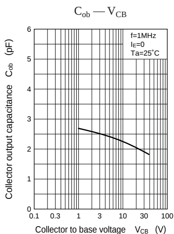
Characteristics charts of UN621F
