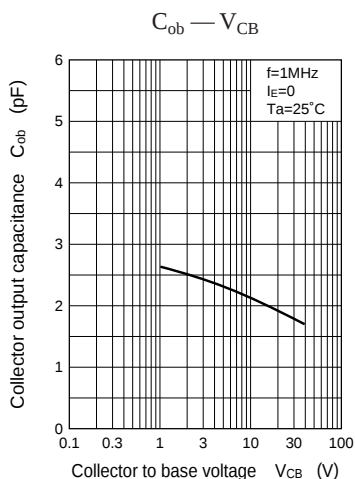
Characteristics charts of UN621E
