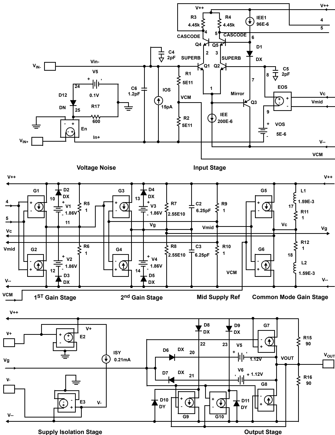
FIGURE 56. SPICE SCHEMATIC
