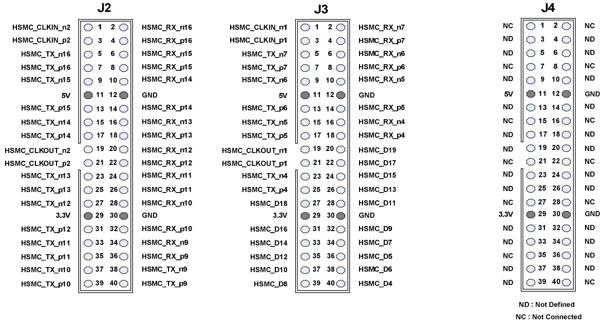
Figure 3.4 Pin-outs of the expansion prototype connectors for Cyclone III Starter board HSMC version
