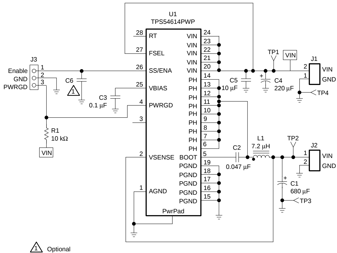
Figure 4–1. EVM Schematic
