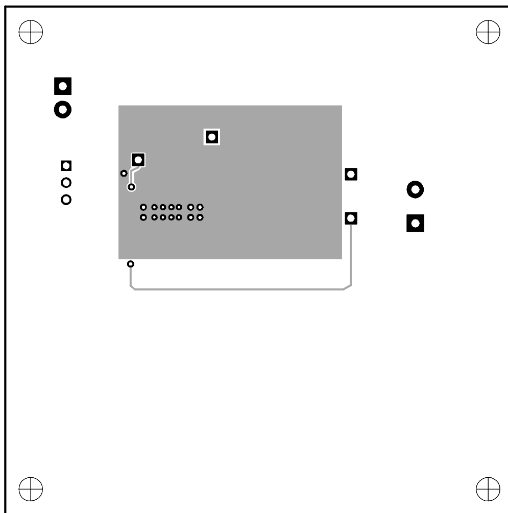
Figure 3–4. Bottom-Side Layout
