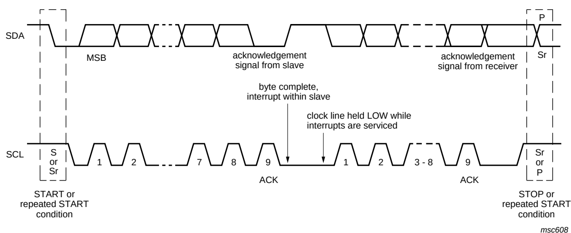
Fig 21. Data transfer on the I 2 C-bus
