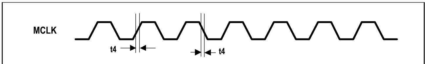
Figure 6. MCLK Timing
