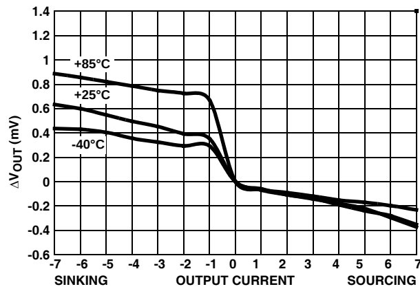
FIGURE 63. LOAD REGULATION
