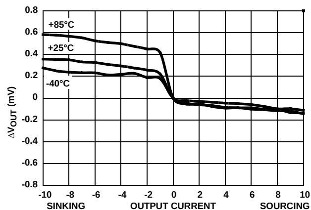
FIGURE 49. LOAD REGULATION
