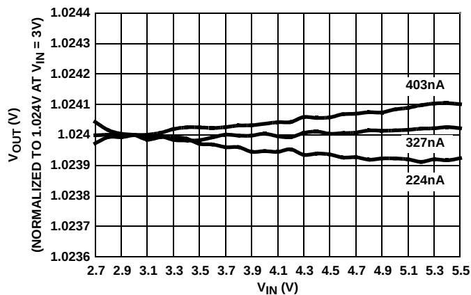
FIGURE 3. LINE REGULATION (3 REPRESENTATIVE UNITS)
