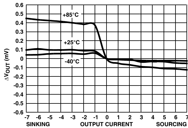
FIGURE 8. LOAD REGULATION
