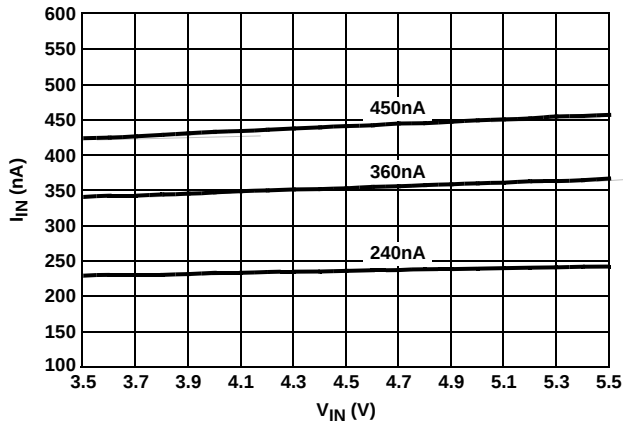
FIGURE 83. I_{IN} vs V_{IN} (3 REPRESENTATIVE UNITS)
