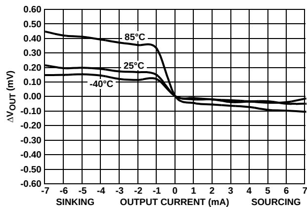
FIGURE 22. LOAD REGULATION
