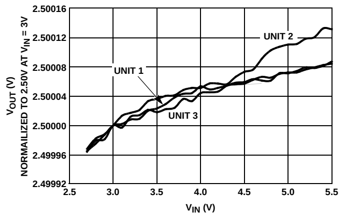
FIGURE 72. LINE REGULATION (3 REPRESENTATIVE UNITS)
