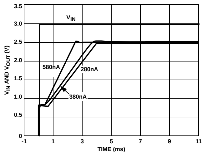
FIGURE 102. TURN-ON TIME
