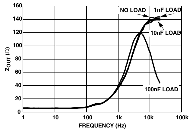
FIGURE 98. Z_{OVT} vs FREQUENCY
