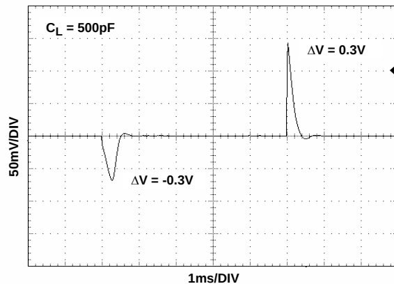
FIGURE 47. NO LOAD LINE TRANSIENT RESPONSE
