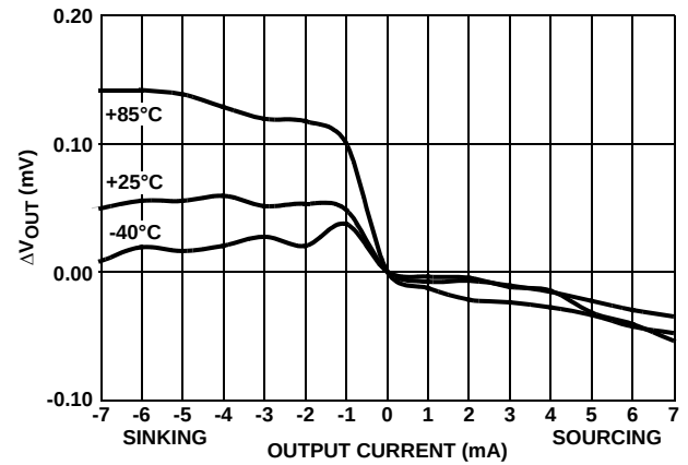
FIGURE 77. LOAD REGULATION
