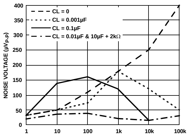
FIGURE 100. NOISE REDUCTION
