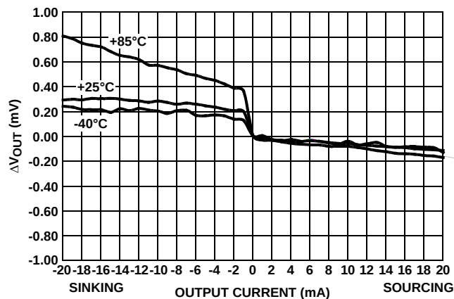
FIGURE 92. LOAD REGULATION I_{SOURCE} - I_{SINK} = \pm 20mA
