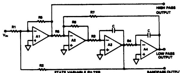
Figure 2. State Variable Filter
