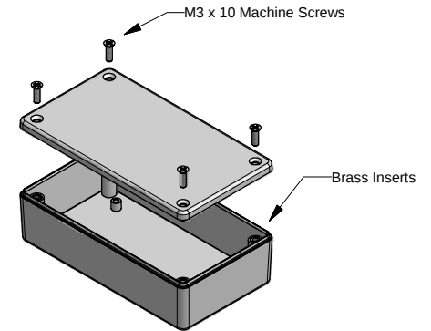
EXPLODED VIEW OF ENCLOSURE
