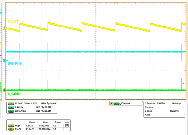
Figure 11. Output ripple, V_{IN} 3.6 V, V_{OUT} 1.8 V, I_{OUT} 10 \mu A
