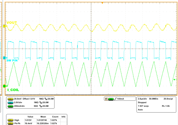
Figure 15. Output ripple, V_{IN} 3.6 V, V_{OUT} 1.8 V, I_{OUT} 250 mA
