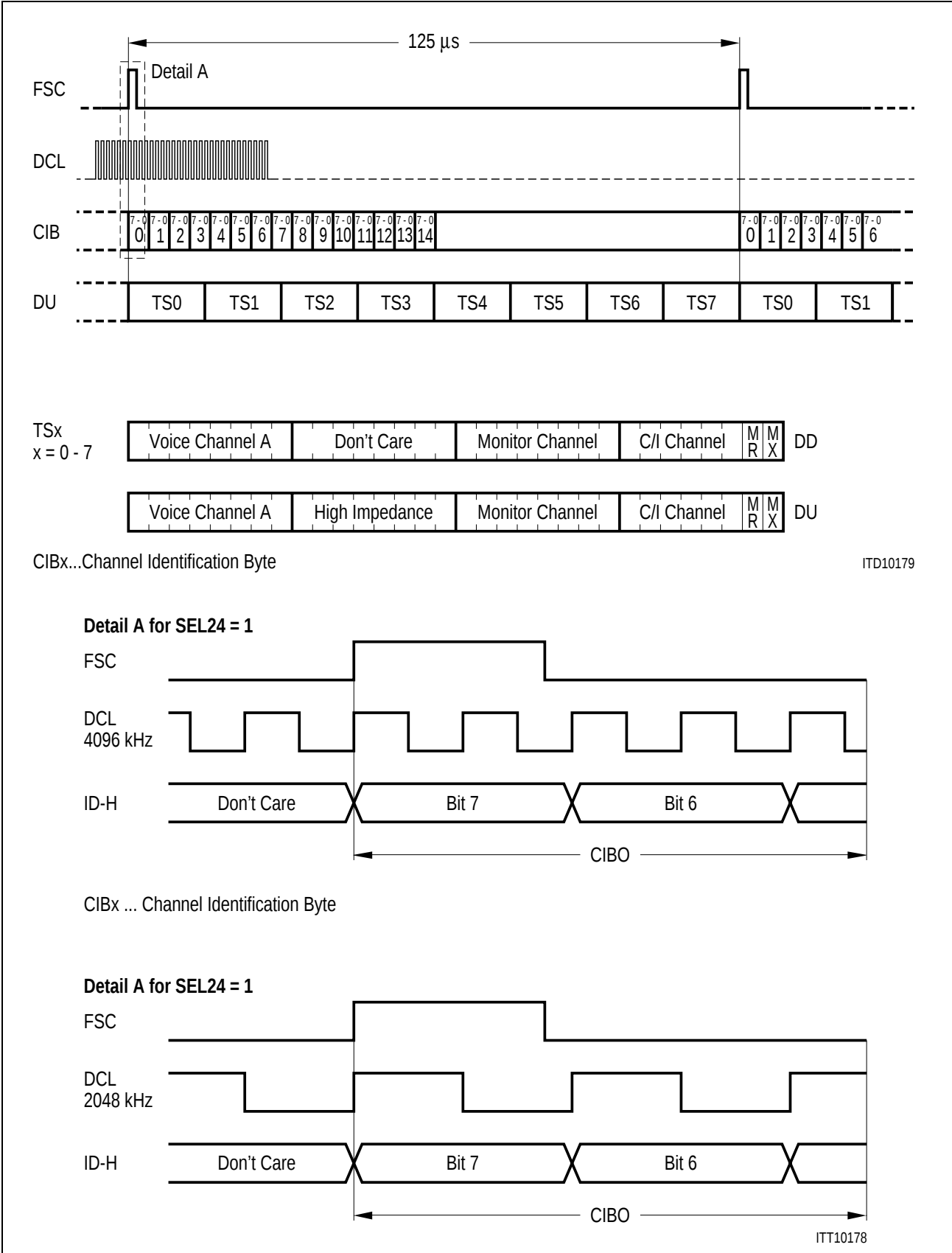
Figure 29 General Timing
