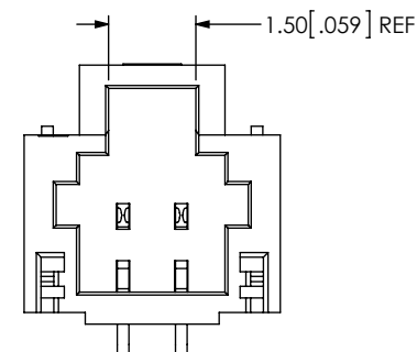
FIG 3 T1M-02-X-SV-L SHOWN (DIFFERENT AS SHOWN, OTHERWISE SAME AS FIG 1) (FOR POSITIONS -02 THRU -04)
