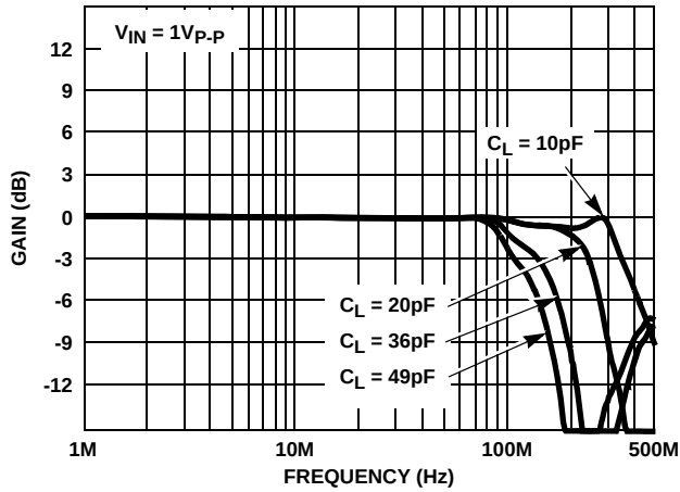
FIGURE 5. FREQUENCY RESPONSE
