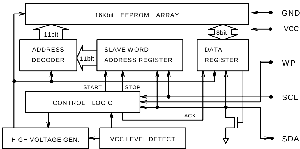
Figure 2. Block Diagram
