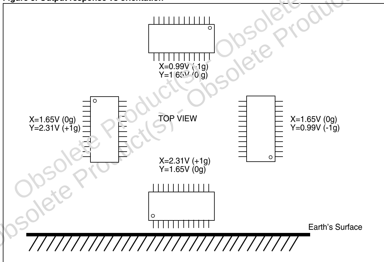
Figure 5 refers to LIS2L02AS4 device powered at 3.3V
