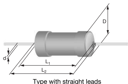
DIMENSIONS - Straight lead type and relevant physical dimensions; see straight leads outline
