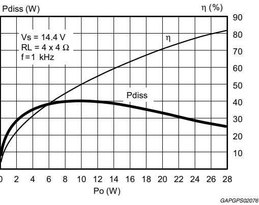
Figure 17. Total power dissipation & efficiency vs. P_o (4 \Omega , Sine)
