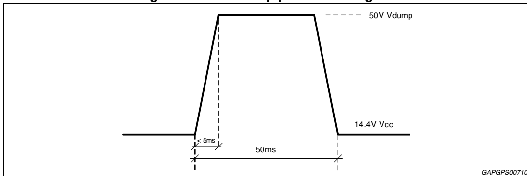
Figure 25. Load dump protection diagram
