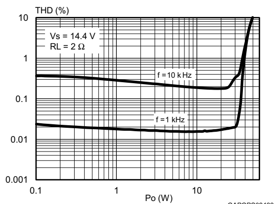
Figure 10. Distortion vs. output power (2 Ω)
