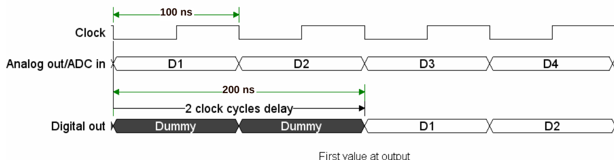
Figure 8. ADC Timing
