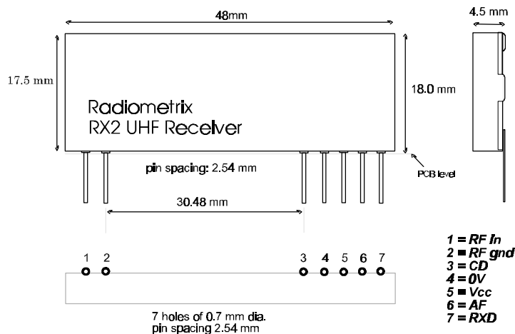
fig. 4: physical dimensions
