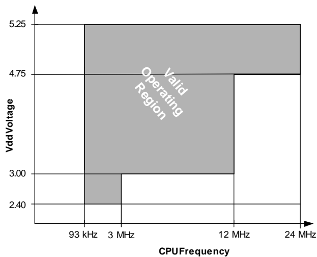
Figure 6. Voltage versus CPU Frequency, and Voltage versus IMO Frequency
