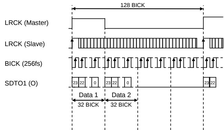
Figure 42. Mode 24/28 Timing (TDM128 mode, MSB Justified, 24-bit)
