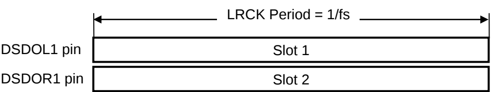
Figure 58. Slot Assign in DSD mode
