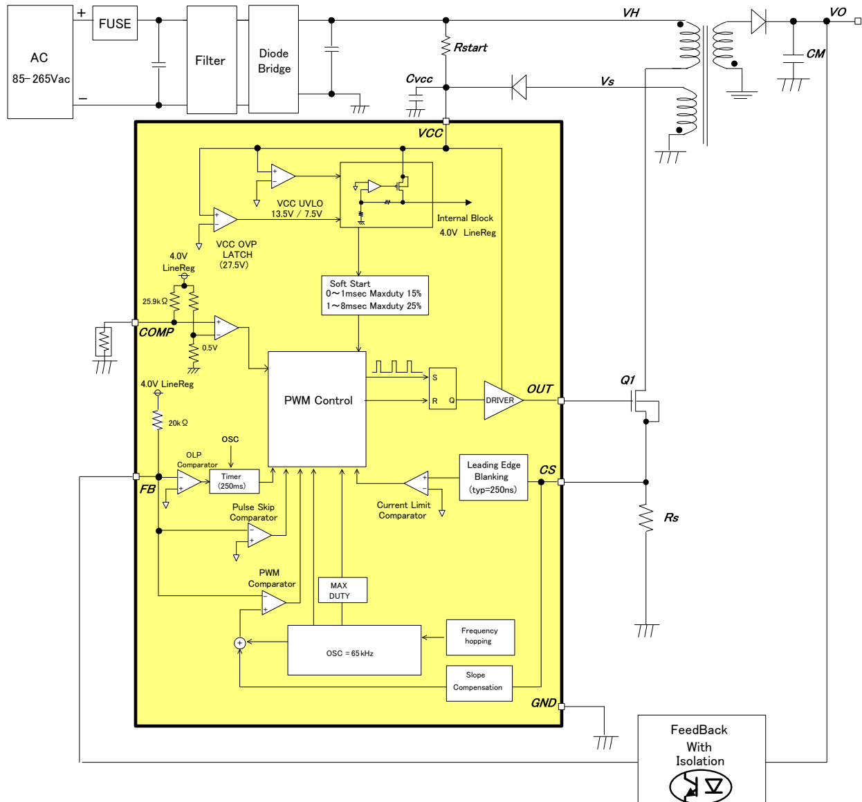
Figure 4. Block Diagram
