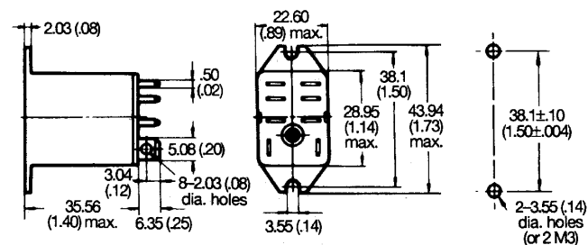
Mounting holes
