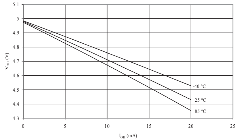
Figure 34-24. ATmega48P/PV: I/O Pin Output Voltage vs. Source Current ( V_{CC} = 5V )
