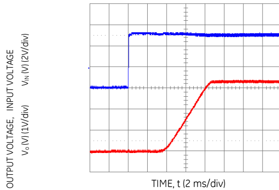
Figure 17. Typical Start-Up with application of V_{in} ( V_{in} = 5.0 Vdc, V_o = 3.3 Vdc, I_o = 5 A).
