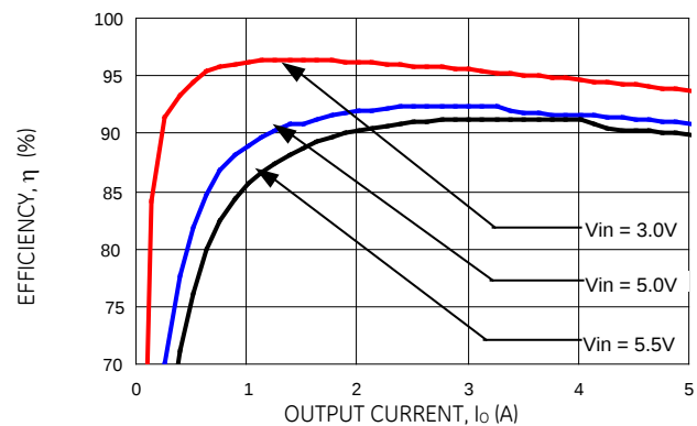
Figure 5. Converter Efficiency versus Output Current (V out = 2.5Vdc).
