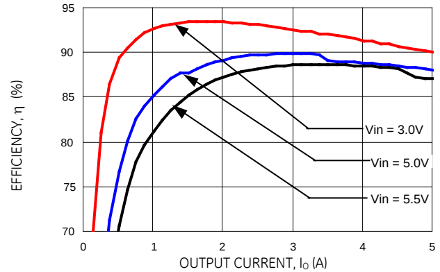
Figure 4. Converter Efficiency versus Output Current (V out = 1.8Vdc).
