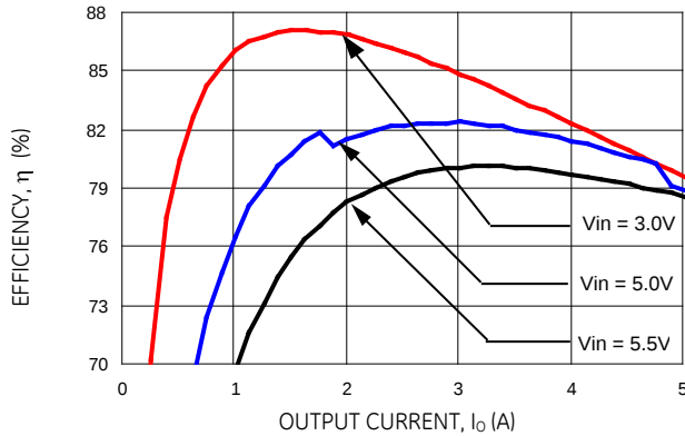
Figure 1. Converter Efficiency versus Output Current (V out = 0.75Vdc).
