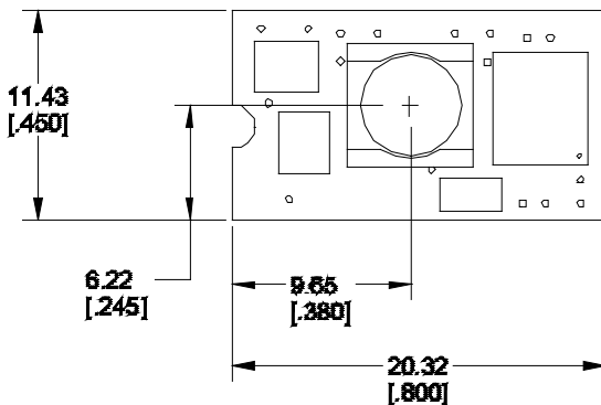
Figure 36. Pick and Place Location.
