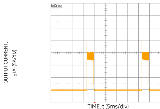
Figure 19. Output short circuit Current ( V_{in} = 5.0 Vdc, V_o = 0.75 Vdc).
