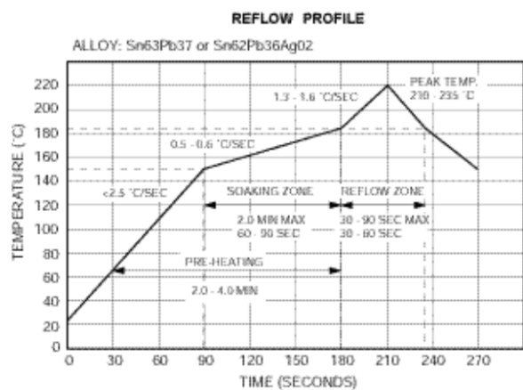
Figure 37. Reflow Profile.
