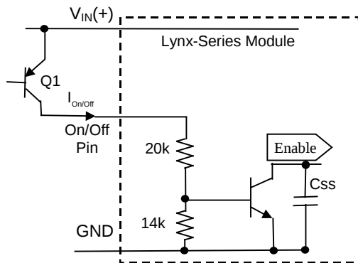
Figure 29. Remote On/Off Implementation.
