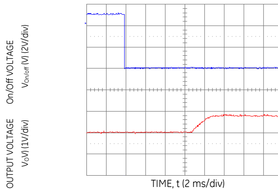
Figure 18. Typical Start-Up Using Remote On/Off with Prebias ( V_{in} = 3.3 Vdc, V_o = 1.8 Vdc, I_o = 1.0 A, V_{bias} = 1.0 Vdc).
