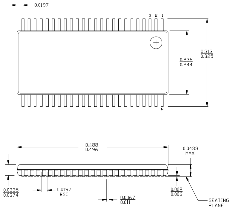
48-Lead Thin Shrunk Small Outline Package Z48
