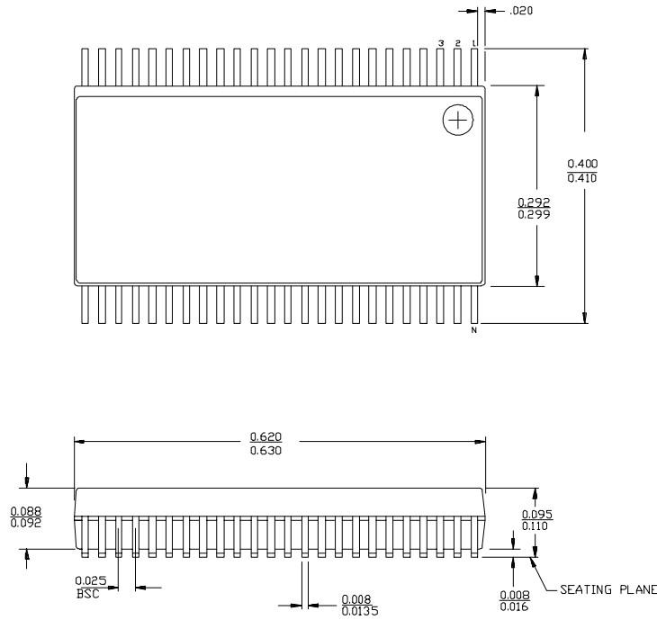
48-Lead Thin Shrunk Small Outline Package Z48
