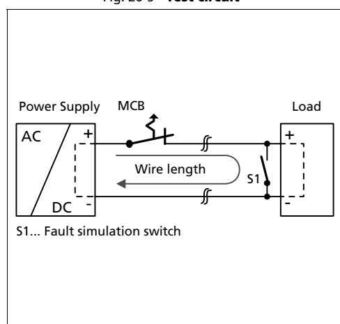
Fig. 26-5 Test circuit
