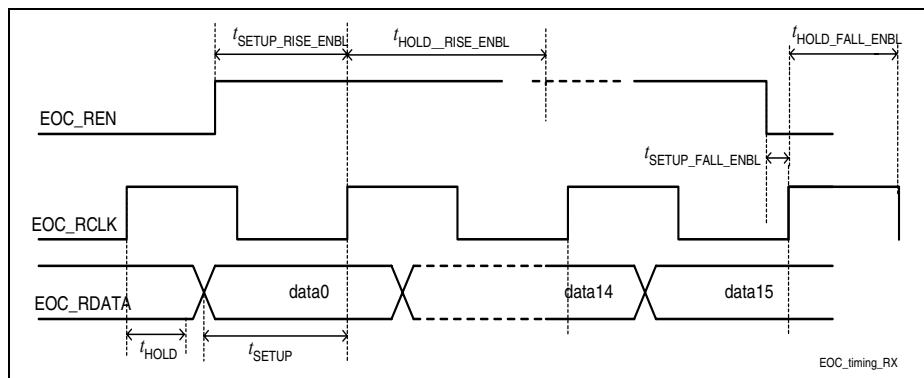
Figure 52 EOC Reception Timing
