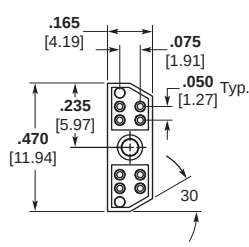
10 Layout
