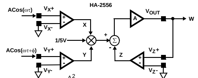
FIGURE 8. PHASE DETECTION
