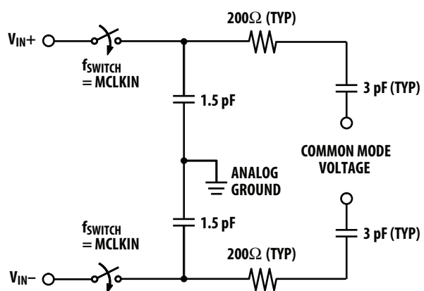
Figure 22. Analog input equivalent circuit.
