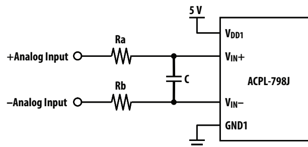
Figure 23. Simplified differential input connection diagram.
