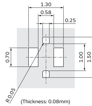
The standard solder cream stencil mask drawing
