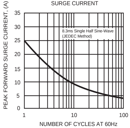
FIG. 2 - MAXIMUM NON-REPETITIVE FORWARD SURGE CURRENT
