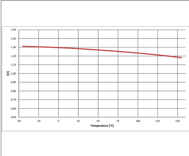
Input Voltage Threshold V_{IN(L)} = f(T_J)
