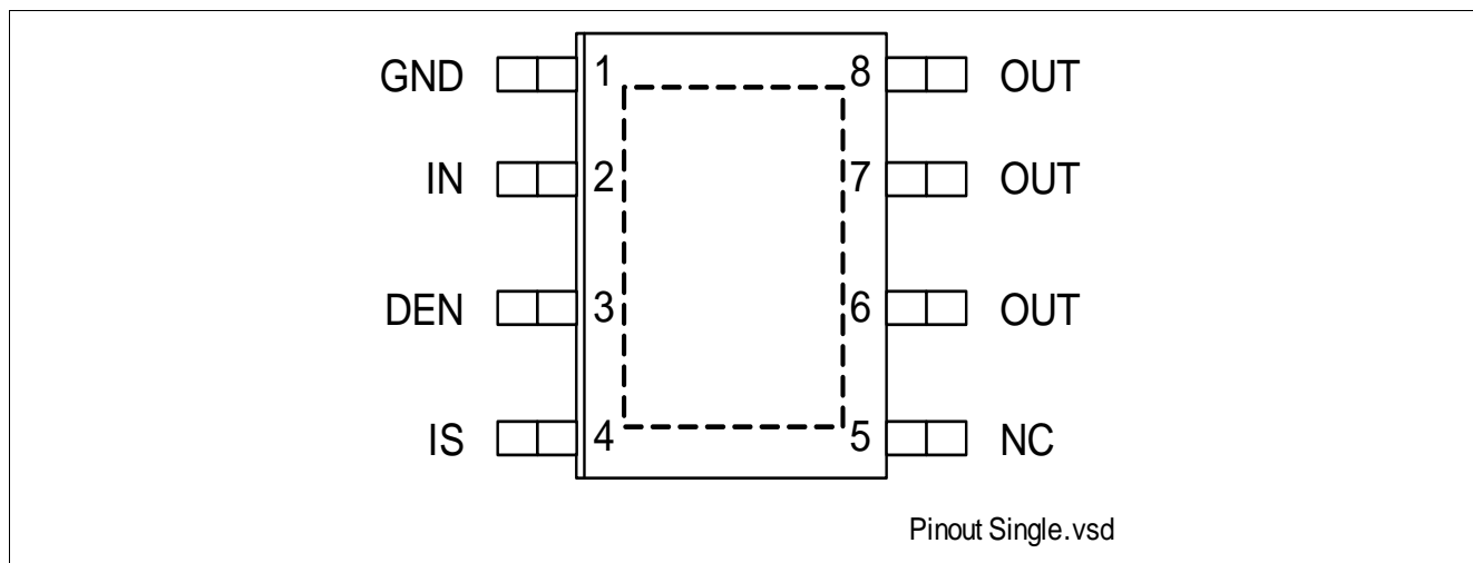
Figure 1 Pin Configuration
