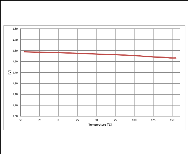
Input Voltage Threshold V_{IN(H)} = f(T_J)
