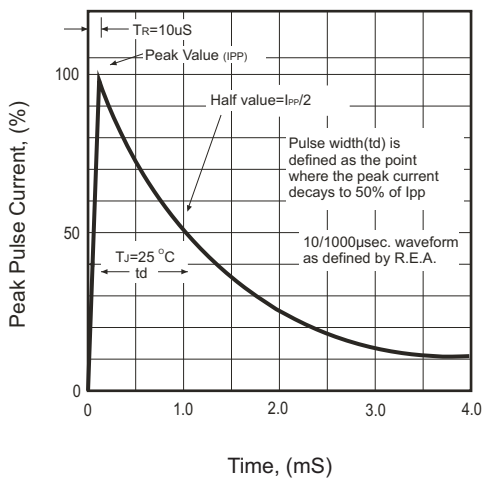
Fig.5 - Pulse Waveform
