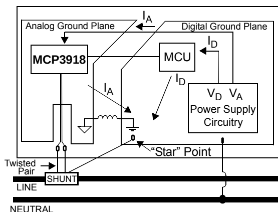
FIGURE 8-5: Connection Diagram.
