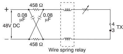
Circuit
