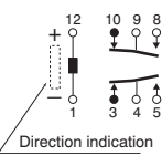
1 coil latching
