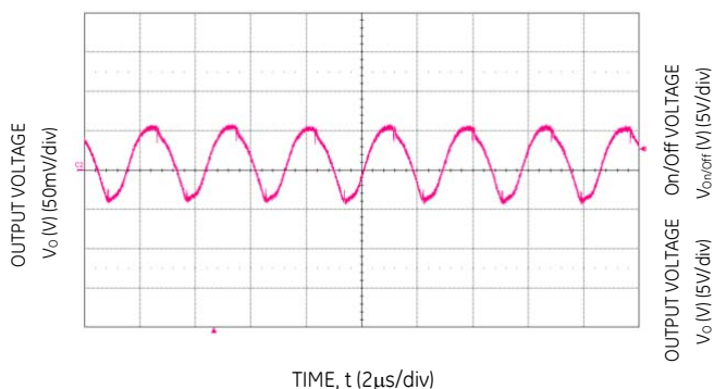
Figure 2. Typical output ripple and noise ( I_o = I_{o,max} ).
