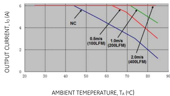
Figure 16a. Output Current Derating for the Module with Heatplate; Airflow in the Transverse Direction from Vout(+) to Vout(-); Vin = 48V.
