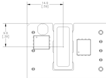
Figure 17. Pick and Place Location.
